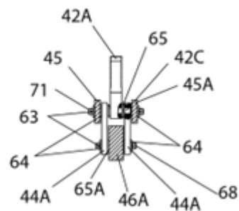
Section N-N
