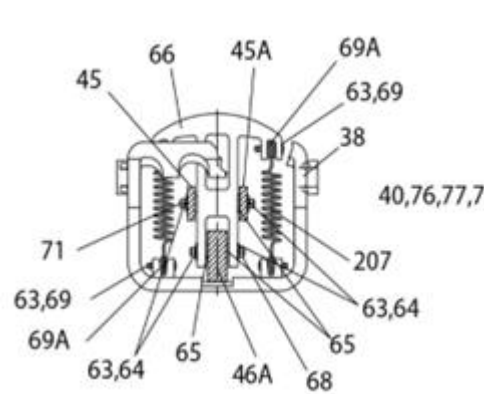
Section J-J
