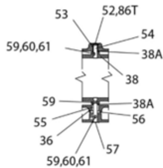
Section K-K
